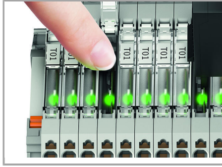
Configuration via push/slide switch
