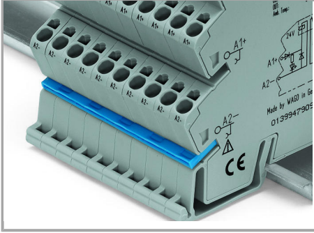
Commoning, not discrete wiring – same outline allows the use of a single in-line, push-in jumper
