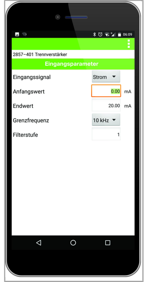
Configuration via WAGO interface configuration app
